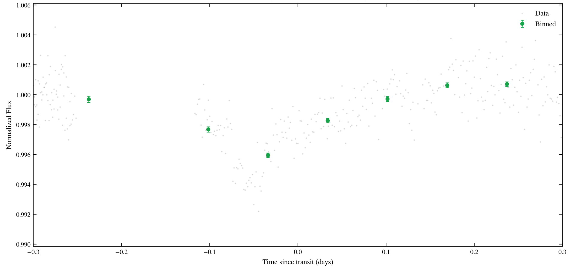
TIC 148914726 | Sectors: 14, 15 | Phase-Folded Transit (P = 13.54761 d)
