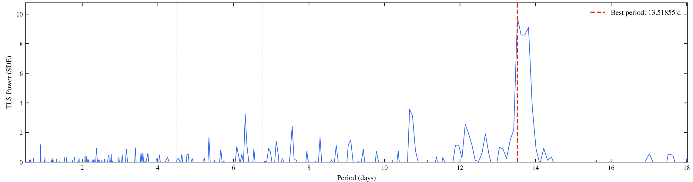
TIC 148914726 | Sectors: 14, 15 | TLS Coarse Periodogram (SDE = 9.78)
