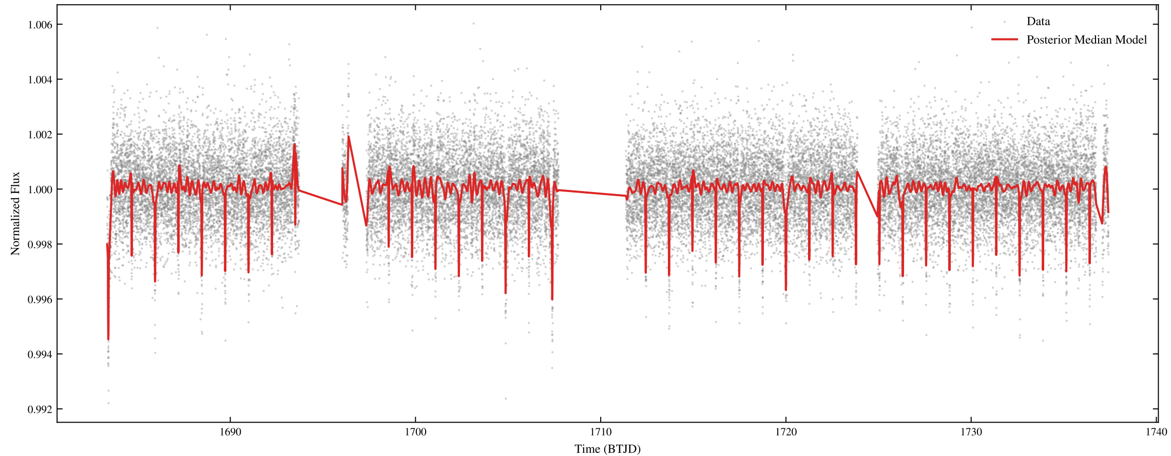
TIC 148914726 | Sectors: 14, 15 | MCMC Posterior Predictive Check
