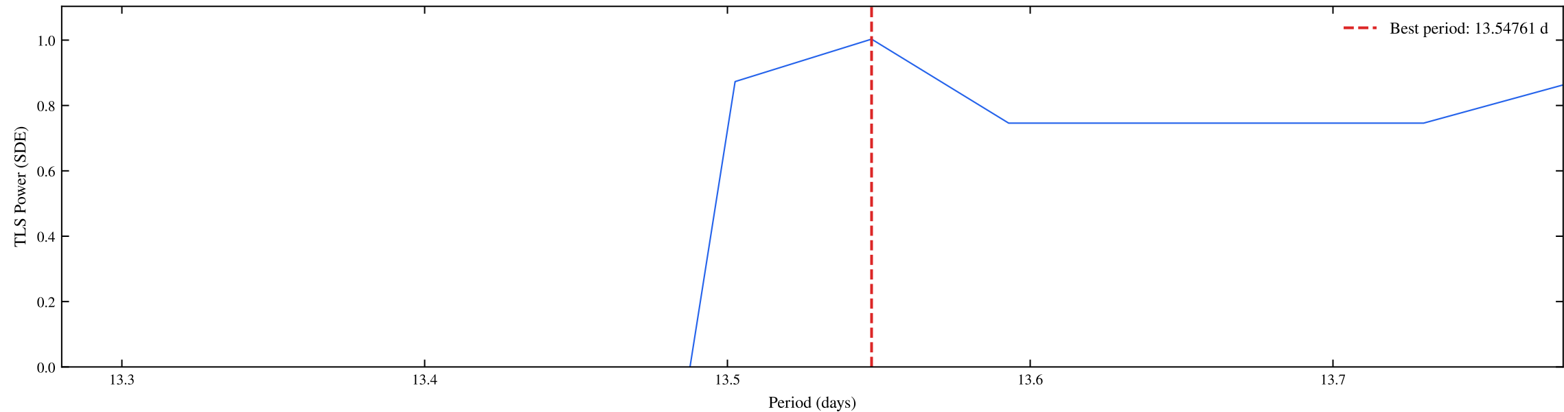
TIC 148914726 | Sectors: 14, 15 | TLS Fine Periodogram (SDE = 1.00)
