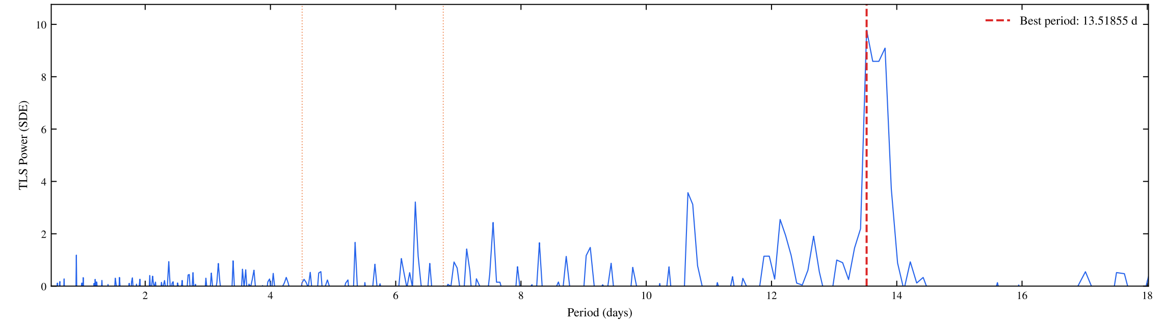
TIC 148914726 | Sectors: 14, 15 | TLS Periodogram (Planet 2 Search) (SDE = 9.78)
