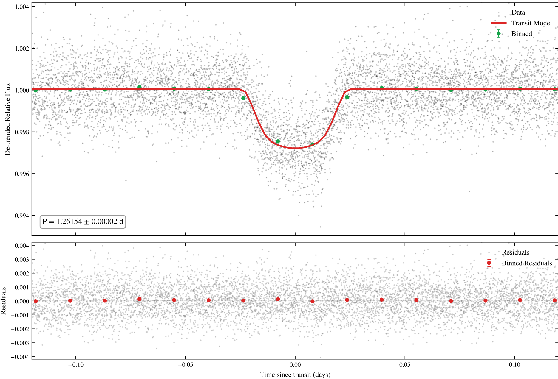
TIC 148914726 | Sectors: 14, 15 | Phased MCMC Fit - Planet 1
