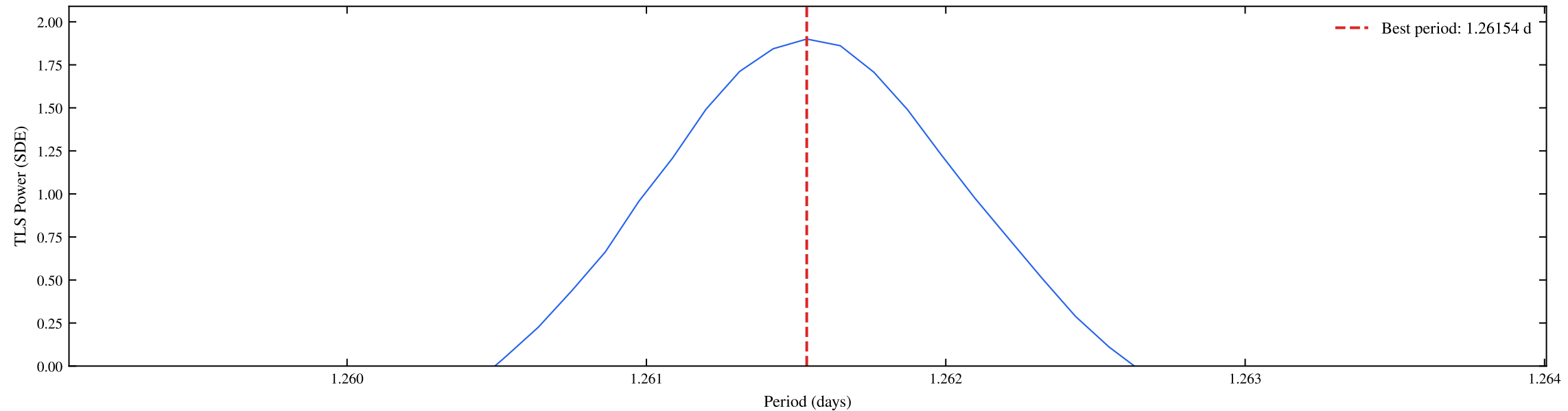
TIC 148914726 | Sectors: 14, 15 | TLS Coarse Periodogram (SDE = 1.90)
