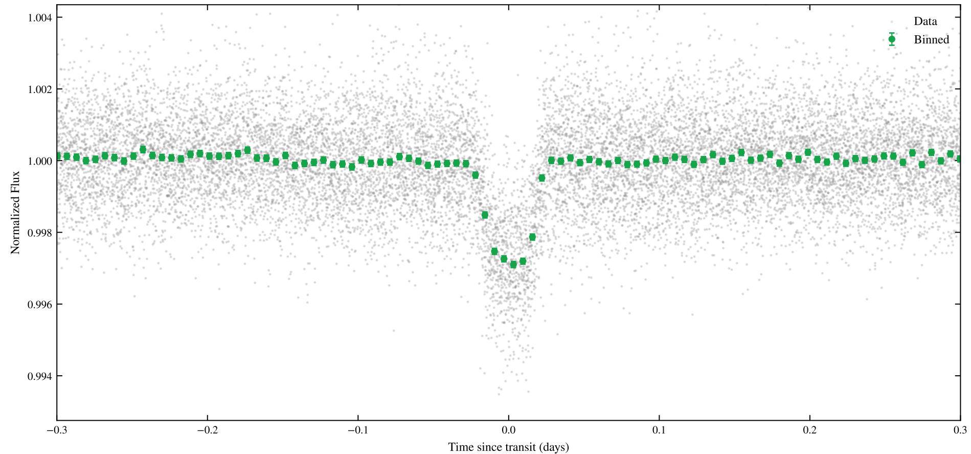
TIC 148914726 | Sectors: 14, 15 | Phase-Folded Transit (P = 1.26154 d)
