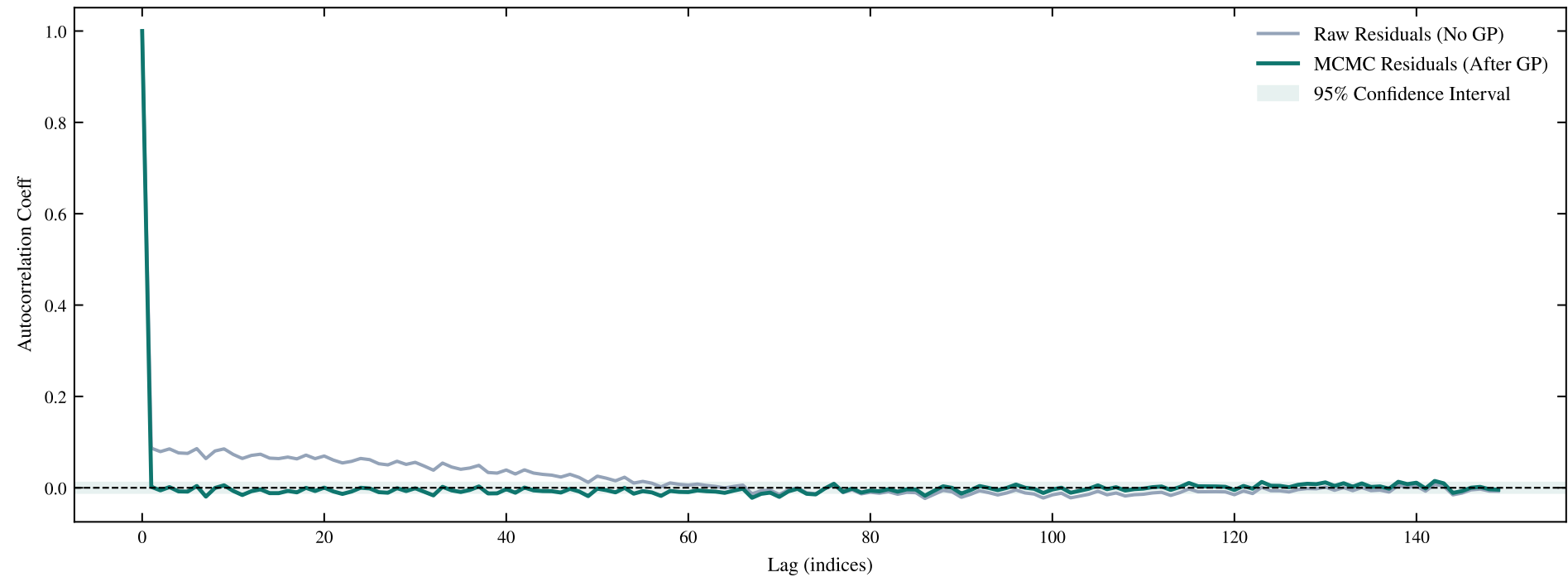
TIC 148914726 | Sectors: 14, 15 | GP Residuals Autocorrelation Function (ACF)
